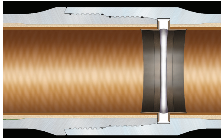
2-Step Connection
