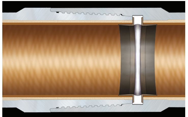
Integral Connection
